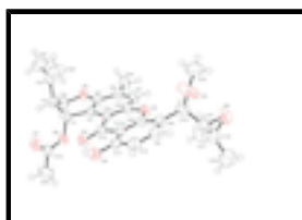
Fig. 1. The molecular structure of the title compound. Displacement ellipsoids are drawn at the 30% probability level. The dashed line indicates a hydrogen bond. Only the major disorder component is shown.
