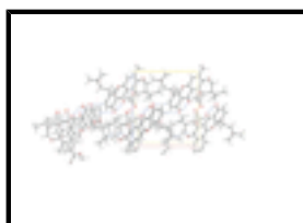
Fig. 2. Molecular packing of the title compound, viewed along b -axis. Hydrogen bonds are shown as dashed lines. Only the major disorder component is shown.
